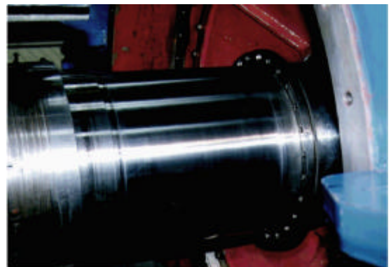
A 533 mm Ø Turbine Journal AFTER Machining and Polishing
